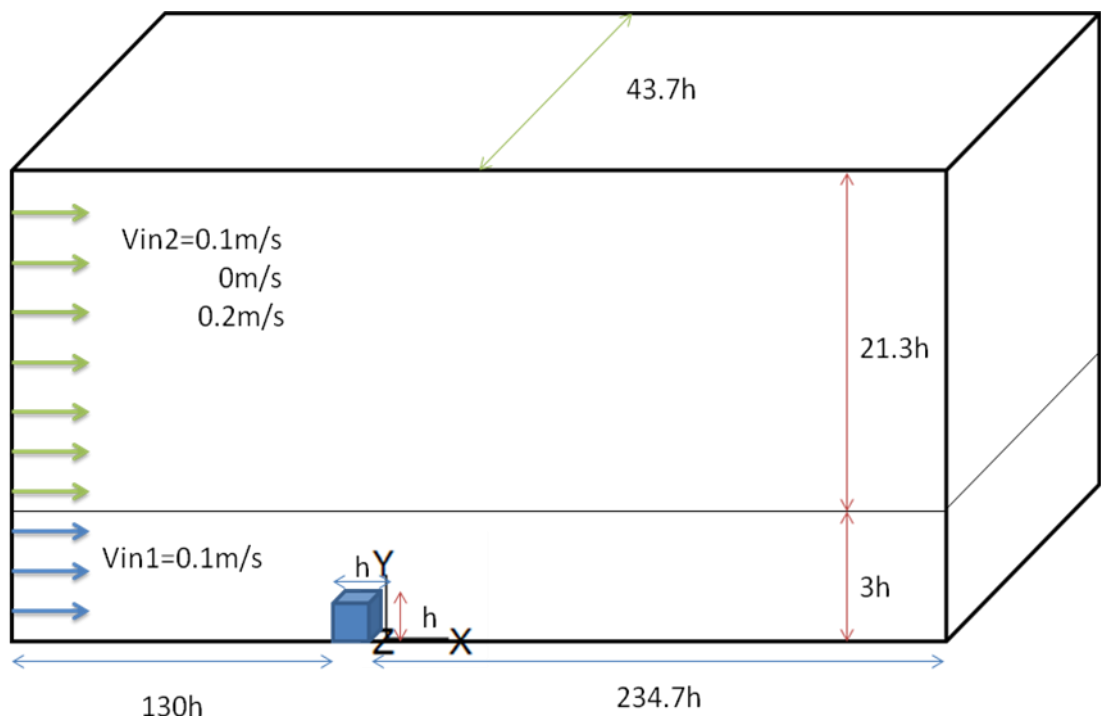
Figure 1: Physical model of the water channel
