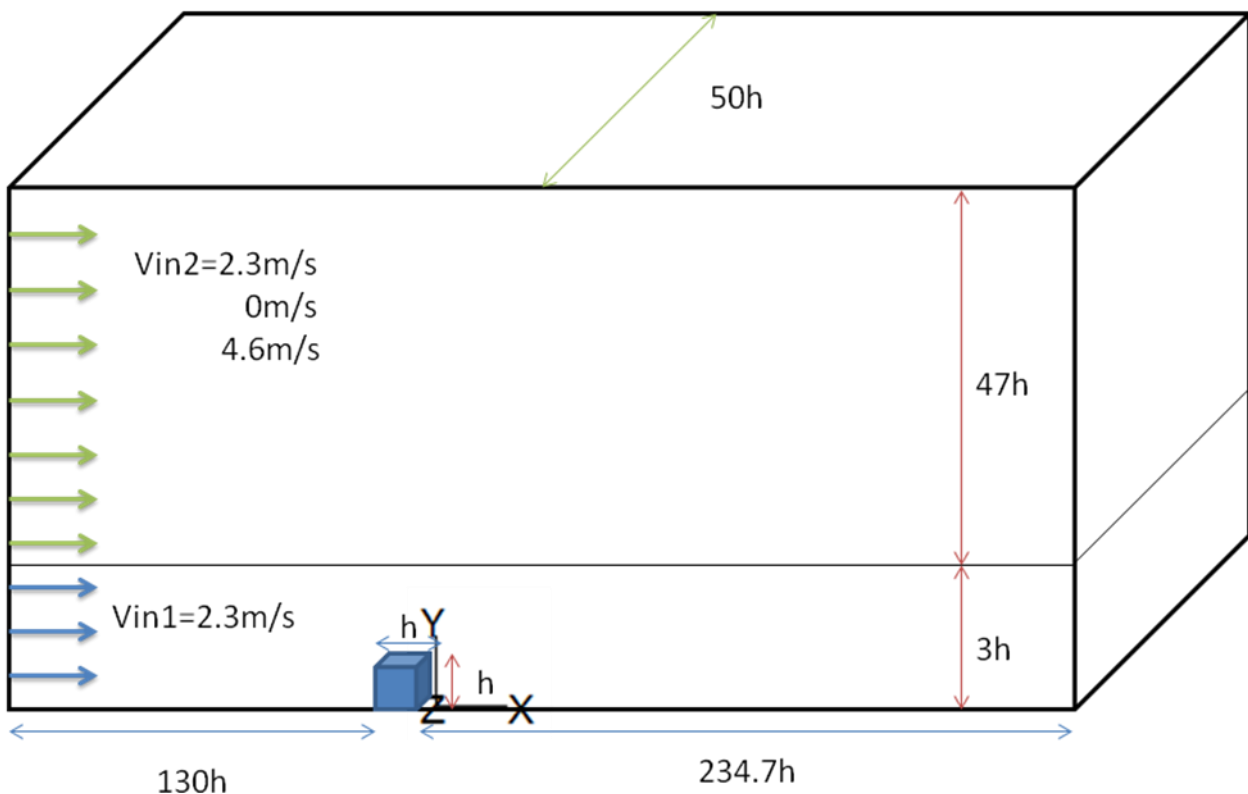
Figure 2: Physical model of the wind tunnel
